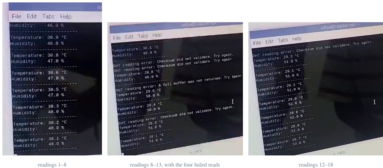
Figure 4: Three frames from the recording of the terminal on the Raspberry Pi while dht.py was running. Each successful read prints a temperature and a humidity line followed by a rule; a failed read prints DHT reading error: with the library’s message — Checksum did not validate when the fifth byte does not match the other four, and A full buffer was not returned when fewer than 40 bits were captured.
